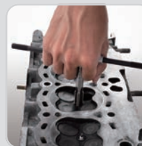
1. Tap re-drilled hole using tap
