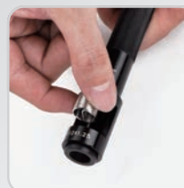
3. Load coiled insert into Coil Shielding Collar
